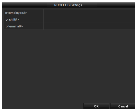
Figure 9-5 NUCLEUS Settings
