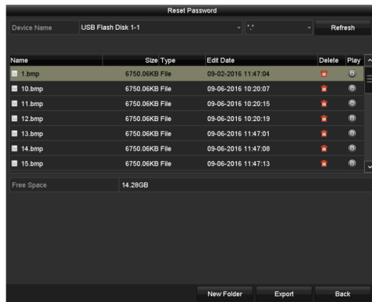
Figure 17-21 Export GUID
