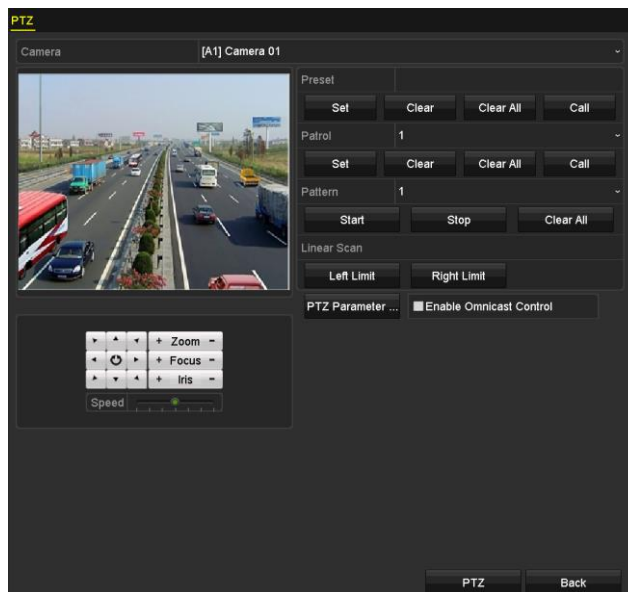
Figure 4-4 PTZ Settings
