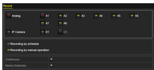
Figure 5-24 Manual Record
