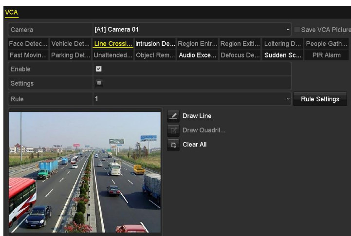
Figure 5-22 VCA Settings
