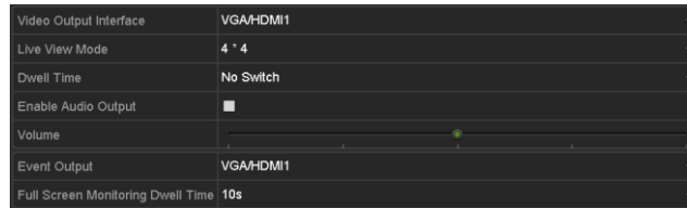
Figure 3-10 Live View-General (1)
