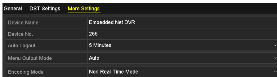
Figure 5-50 More Settings
