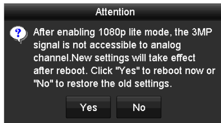
Figure 5-46 Attention
