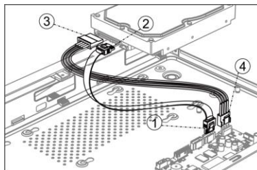
Figure 2-10 Connect Cables
